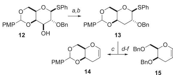
Scheme 4. Synthesis of 3-Deoxygalactal Derivatives a
