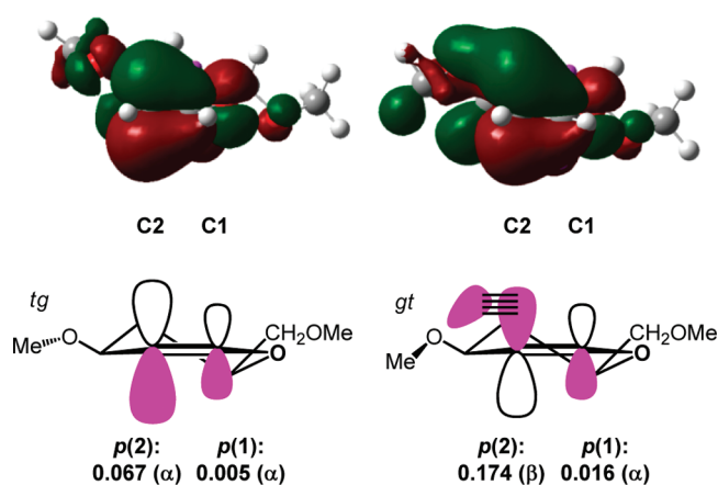
Figure 3. Electron density maps of the 4-deoxyglucal derivative (analogue of 11 ) with the C3 methyl ether in the tg conformation (left) or the gt conformation (right). In the case of gt , the electron density map reveals an incidental (but superfluous) hyperconjugation between the hybrid orbital at C2 and a lone pair on O3 (extended green lobe), creating an artificial polarization in the \beta direction.
