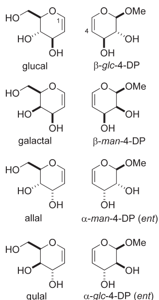
Figure 1. Four diastereomeric glycols, and their 4-deoxypentenoside isosteres.
